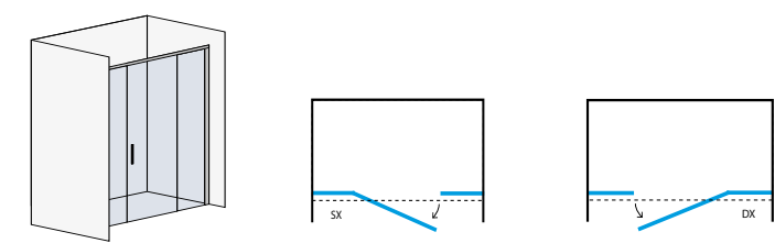
Porta battente + 2 fissi - finitura cromo, nichel, bianco opaco, nero opaco Pivot door + 2 fixed glasses - chrome, nickel, matte white, matte black finishes
