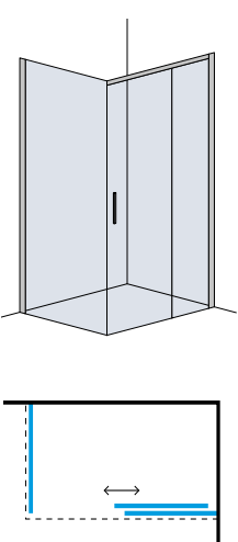
Porta scorrevole + Parete fissa Sliding door + Fixed glass
